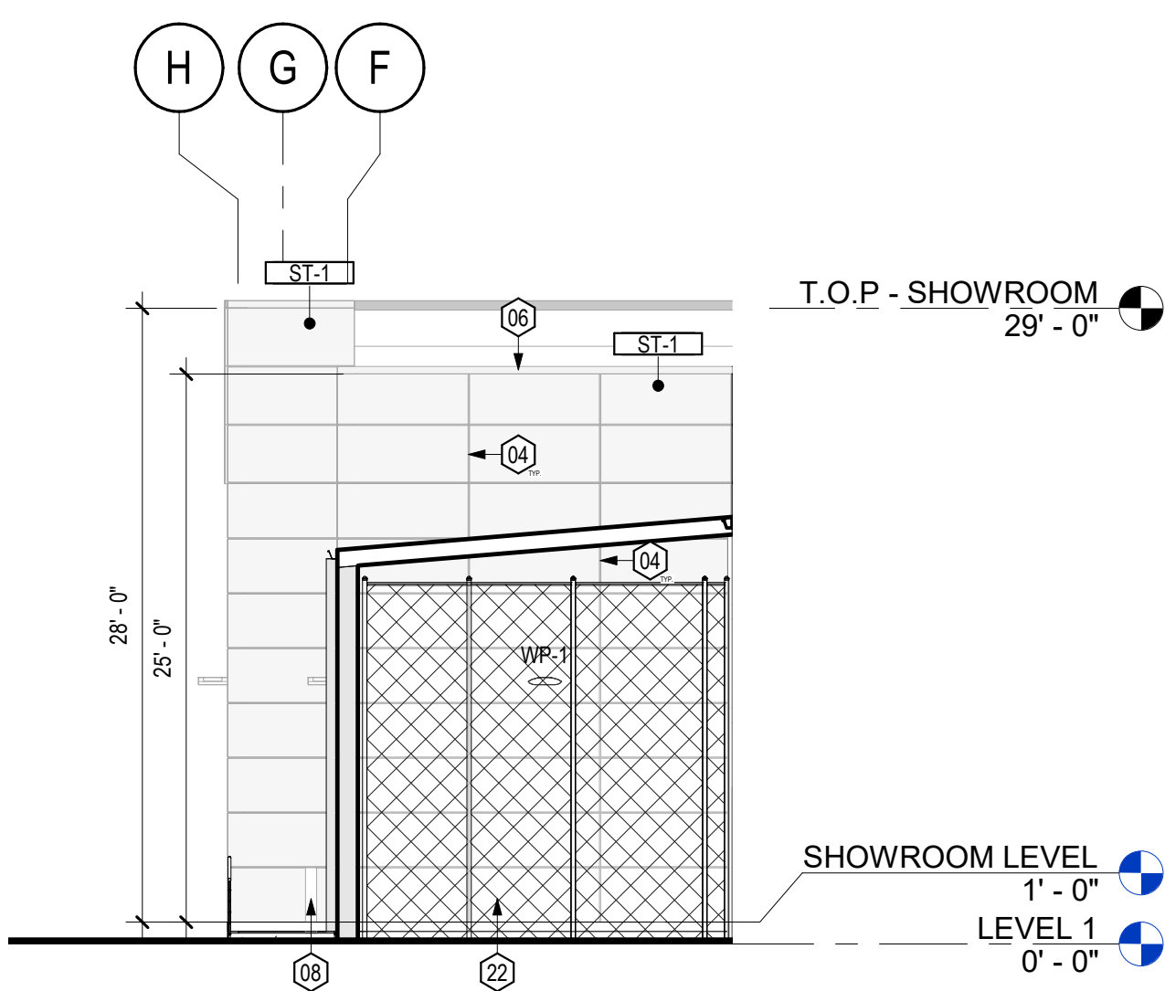
6 EXTERIOR BUILDING ELEVATION @ NVD - SOUTH 1/8" = 1'-0"
