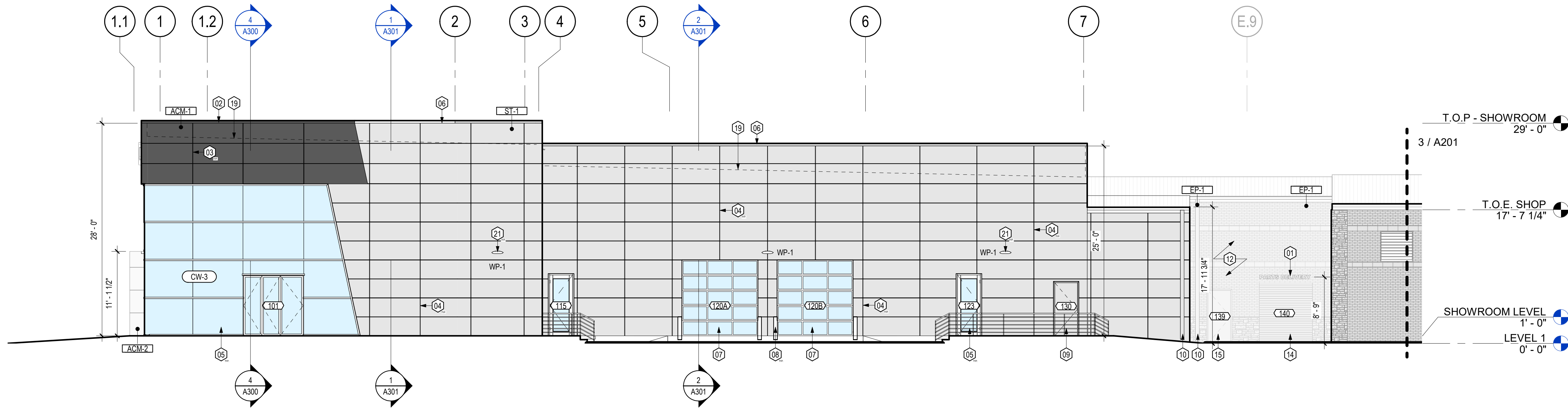
2 EXTERIOR BUILDING ELEVATION - WEST - AREA A 1/8" = 1'-0"
