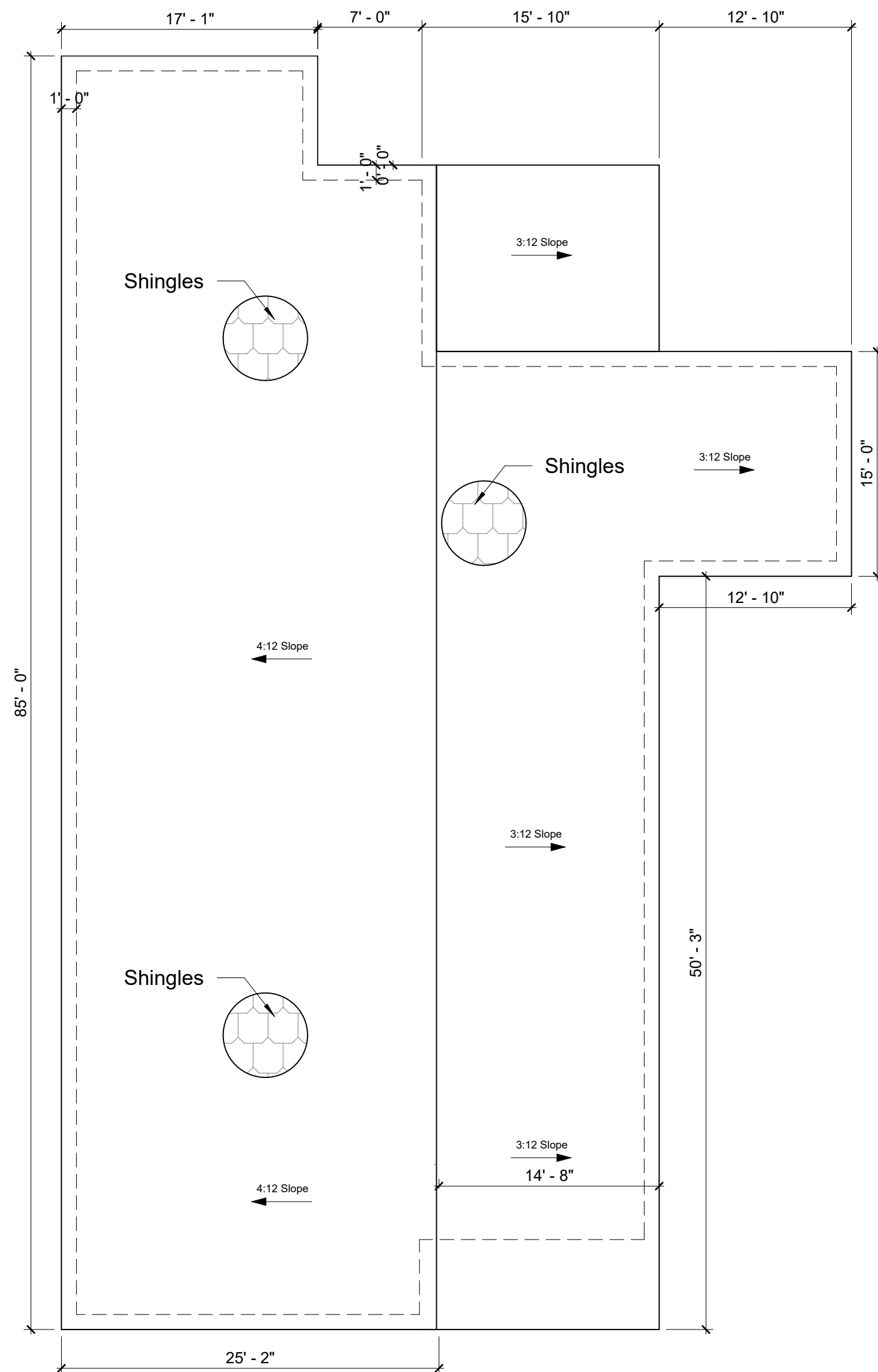
1 Roof 1/8" = 1'-0"
