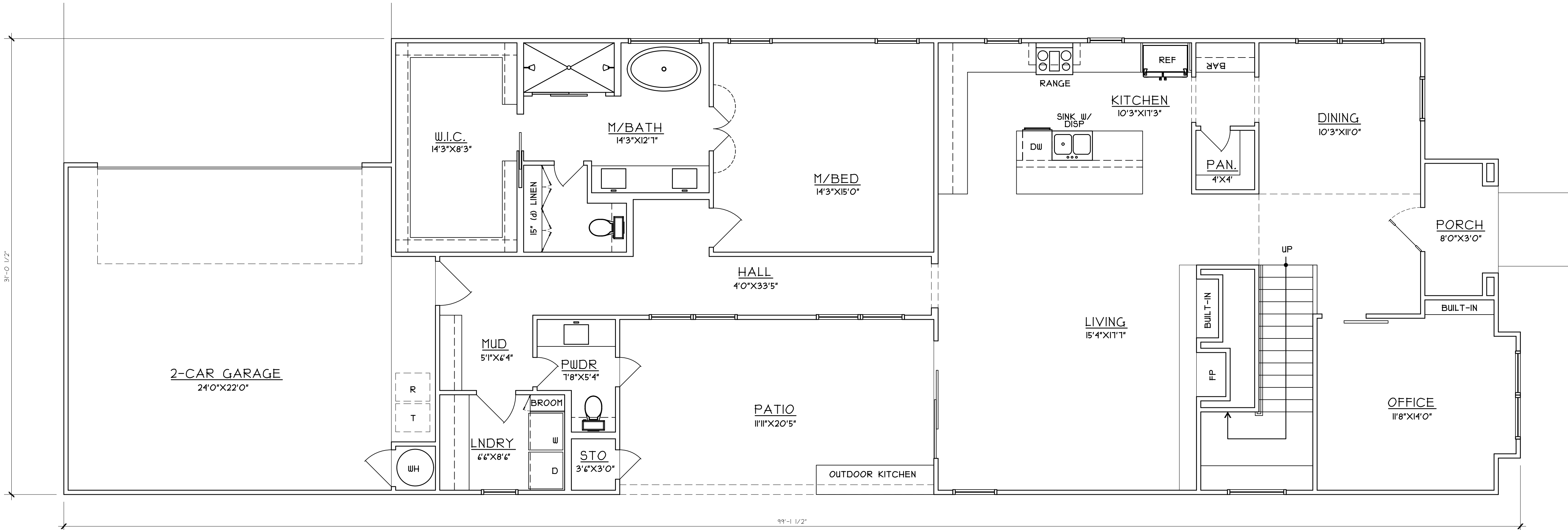
1 FIRST FLOOR PLAN Scale: 1/4" = 1'-0"
