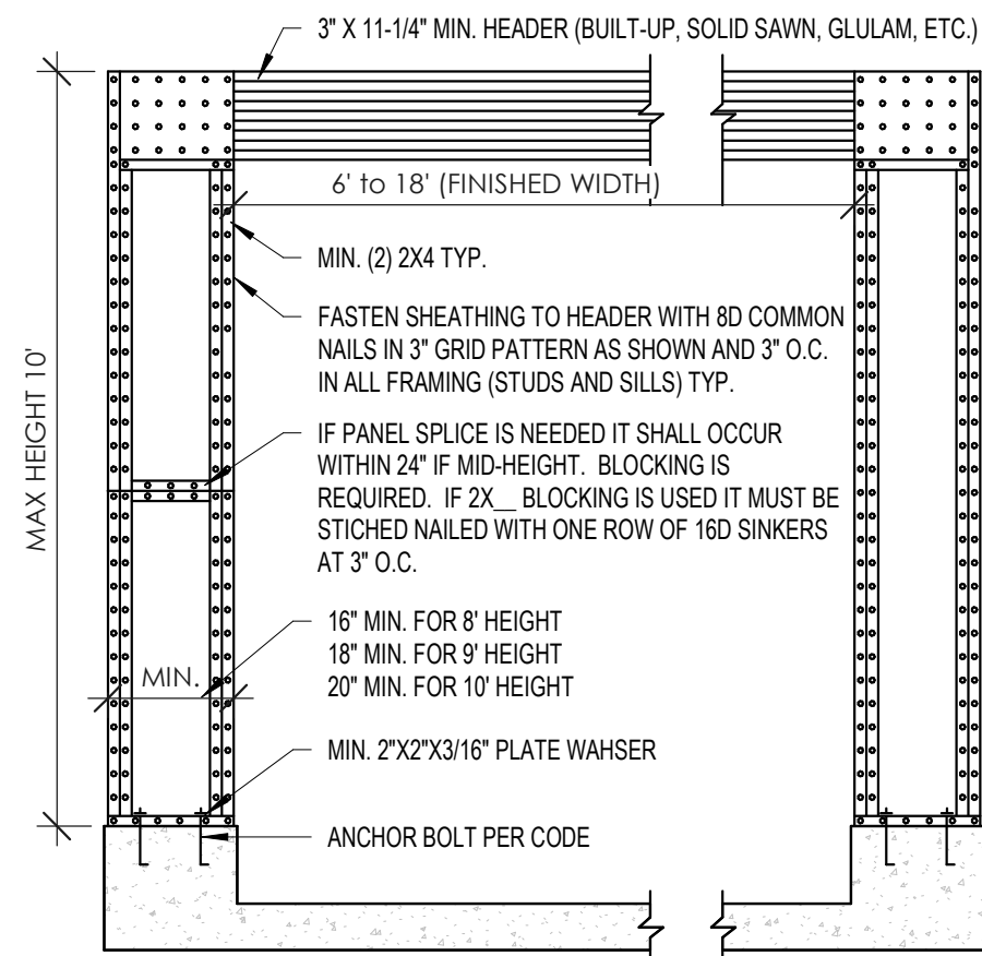
OUTSIDE ELEVATION
