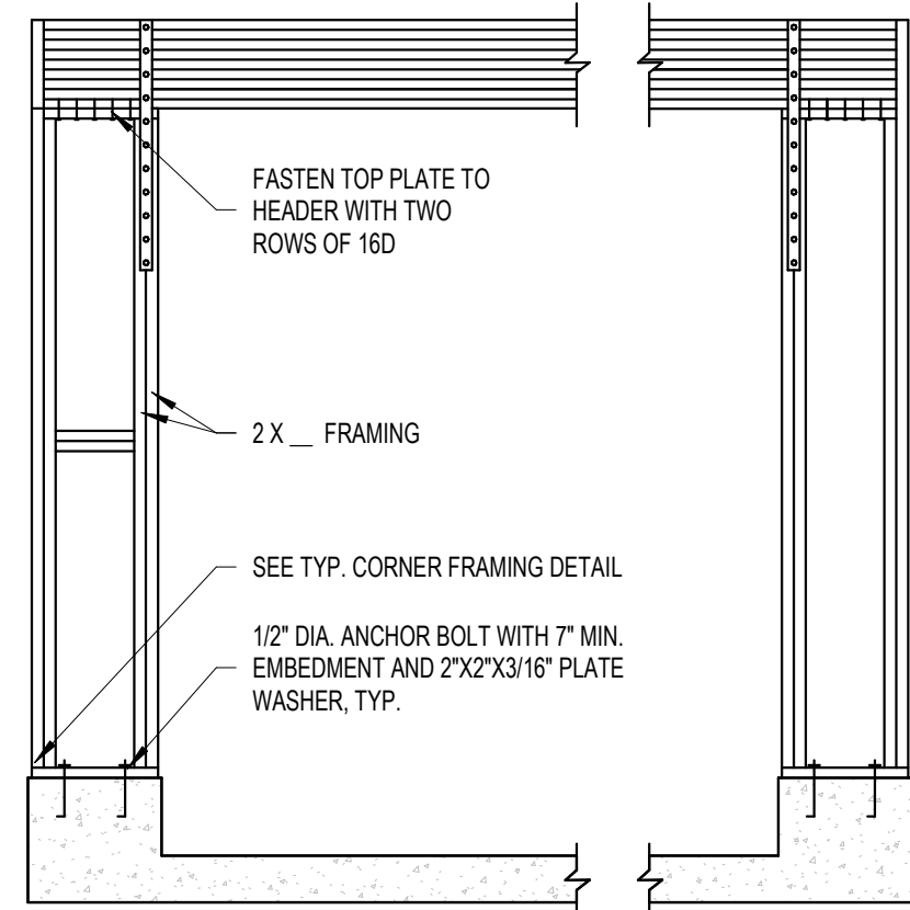
INSIDE ELEVATION
